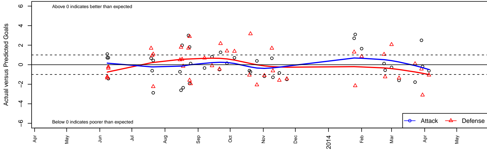
Snohomish United Black B02 Dots are actual minus expected GF (blue circles) and GA (red triangles). Blue line is smoothed change in attack strength. Red is smoothed change in defense strength.
